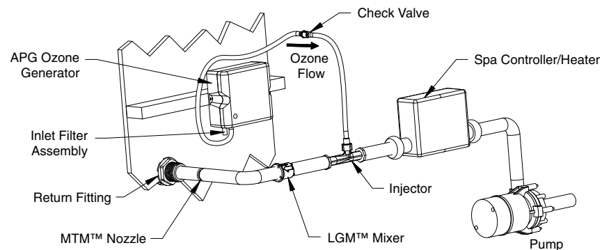
Figure 2: DEL Optimized Mixing System
